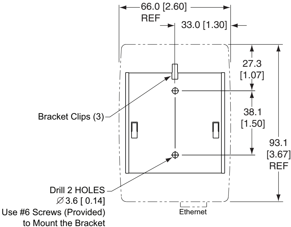
Figure 2.6a Mounting the Coordinator
